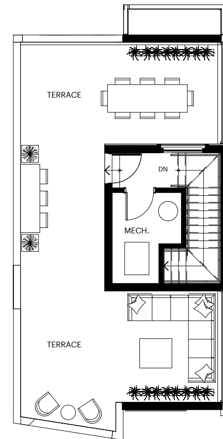
ROOF PLAN
